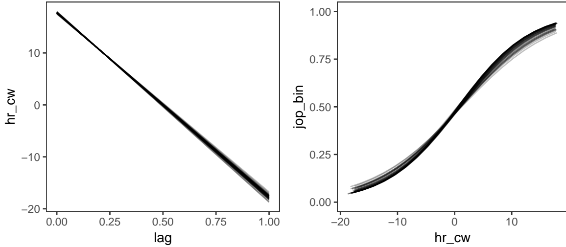
Figure 9. ( #fig:spaghetti-plot-b-binary-y ) Fitted values of the multilevel mediation model with a binary Y , for every individual in the study. Left panel: Subject-specific regression lines for path a. Right panel: Subject-specific fitted values for path b in probability space.
