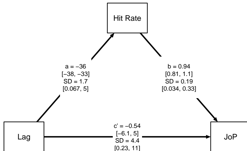
Figure 4. (#fig:example1-path-plot) Path diagram with point estimates (posterior means) of the parameters and associated 95 percent Credible Intervals (in square brackets below the point estimates). Under each estimated average effect, “SD” shows the associated effect’s standard deviation, which indicates the degree to which that effect varies between people (in standard deviation units).
