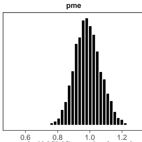
Figure 10. ( #fig:example1-pme-plot ) MCMC samples from the posterior distribution of the population-level proportion of effect that is mediated.
