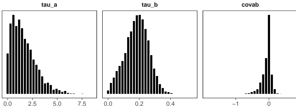
Figure 5. ( #fig:example1-pop-hist ) Histograms of the marginal posterior distributions of the standard deviations of a and b (left, middle), and the a - b covariance (right). Quick visual inspection tells us that these distributions are unlikely to be Gaussian, and therefore using the distributions' means or standard deviations as numerical summaries may be misleading. It is better to interpret the entire distribution.
