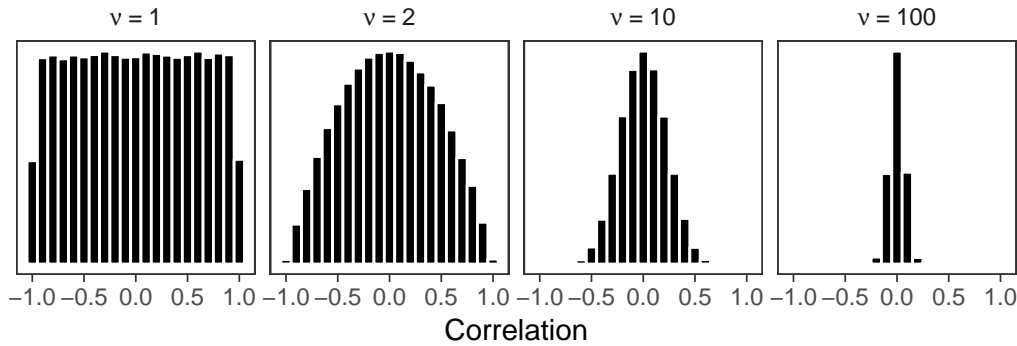
Figure 3. (#fig:lkj-prior-example) Histograms of 100000 random draws from the LKJ prior distribution for four values of \nu .
