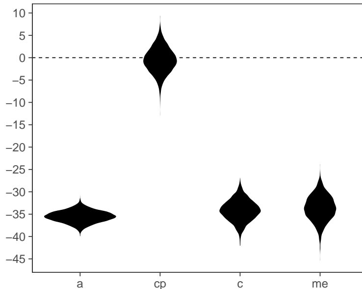
Figure 6. (#fig:example1-pop-violin) Violin plots of the estimated parameters. Each dark violin shape is a mirrored top-down view of a density plot.
