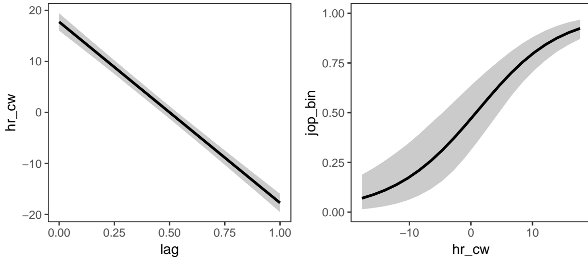
Figure 8. ( #fig:spaghetti-plot-binary-y ) Fitted values of the multilevel mediation model with a binary Y. Left panel: Population-level regression line for path a and its 95%CI as a grey shade. Right panel: Population level regression line for path b in probability space, and its 95%CI.
