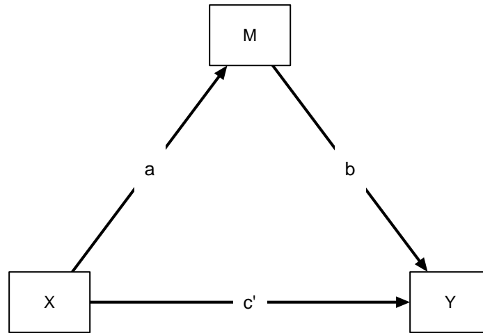
Figure 1. (#fig:template-mediation-plot)Diagram of the mediation model.
