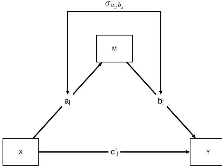
Figure 2. (#fig:template-multilevel-mediation)Diagram of the within-subjects mediation model.
