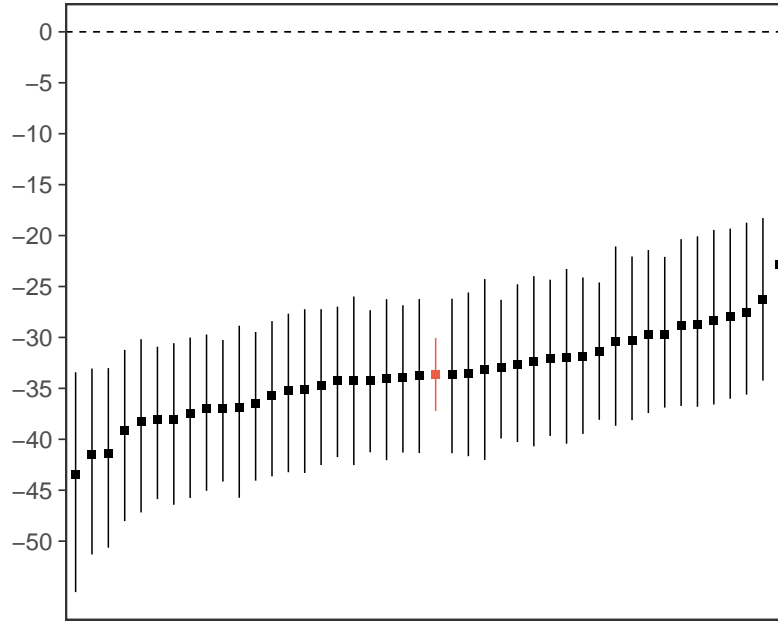
Figure 7. ( #fig:example1-subj-coefs ) Coefficient plot of the person-level estimates of the mediation effect. Each square represents the mean of an individual's estimated ab parameter, and the lines cover the 80% CI of the parameters. By adjusting the “ pars ” argument, we also include the average level estimate, which is automatically displayed in red.
